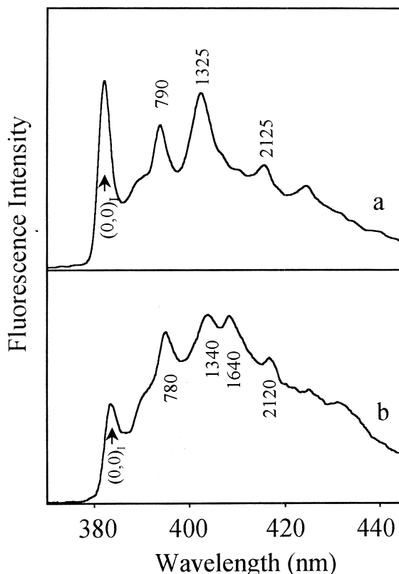
Fig. 7. On-line NLN spectra (a and b) for the CE-separated peaks 7 and 11 of Fig. 6. The bands are labeled with their ground-state vibrational frequencies, in \text{cm}^{-1} ; T=4.2\text{ K} , \lambda_{\text{ex}}=308\text{ nm} .
