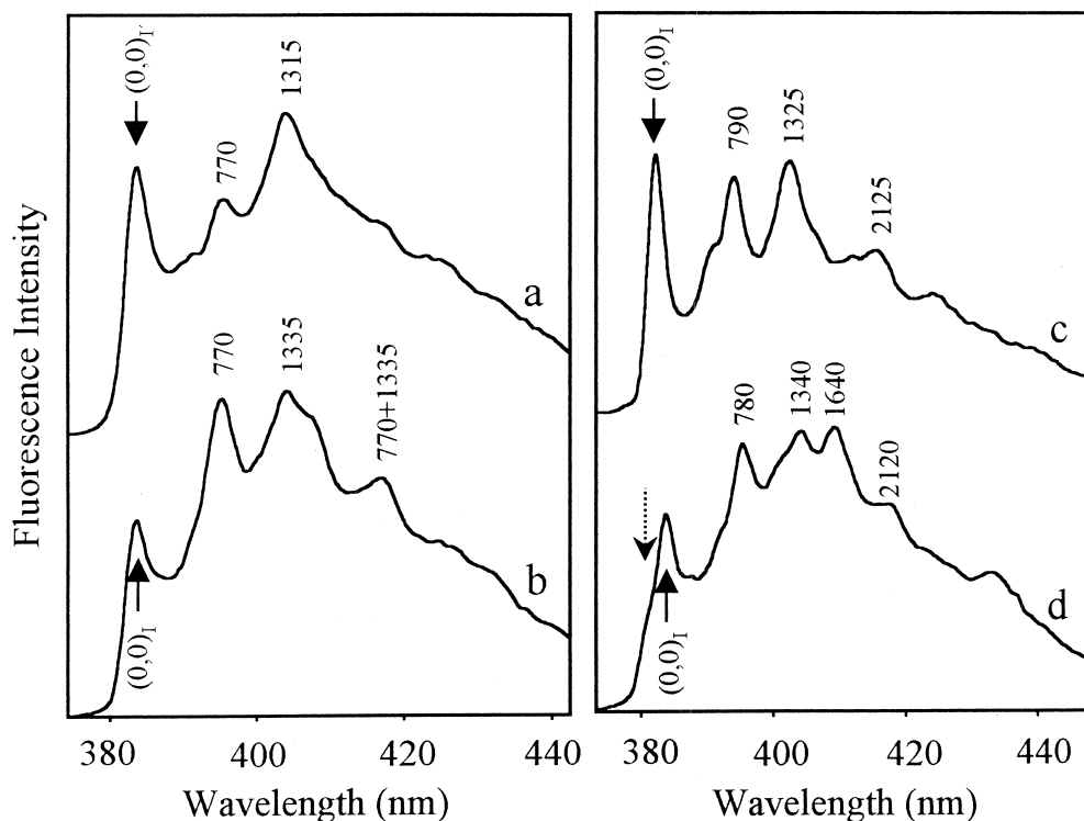
Fig. 3. NLN fluorescence spectra obtained off-line for (–)- trans-anti -DB[ a,l ]PDE-14-N 6 dA (spectrum a), (–)- cis-anti -DB[ a,l ]PDE-N 6 dA (spectrum b), (+)- trans-syn -DB[ a,l ]PDE-14-N 6 dA (spectrum c), and (+)- cis-syn -DB[ a,l ]PDE-N 6 dA (spectrum d) adducts in CE buffer. T=4.2 K, \lambda_{ex}=308 nm, delay time=80 ns, and gate width=200 ns. The numbers correspond to the ground state ( S_0 ) vibrational frequencies.
